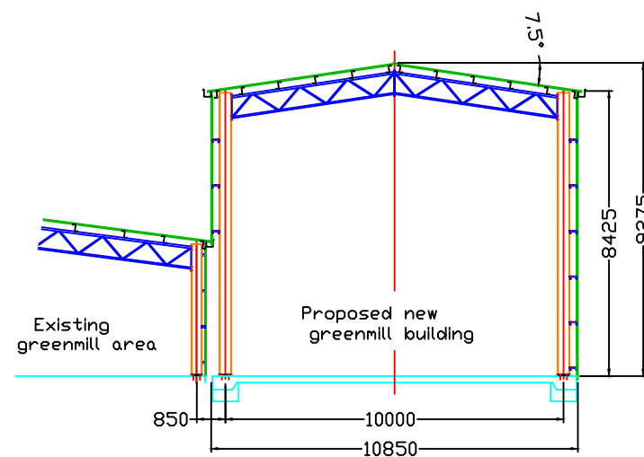
SECTIONAL VIEW
