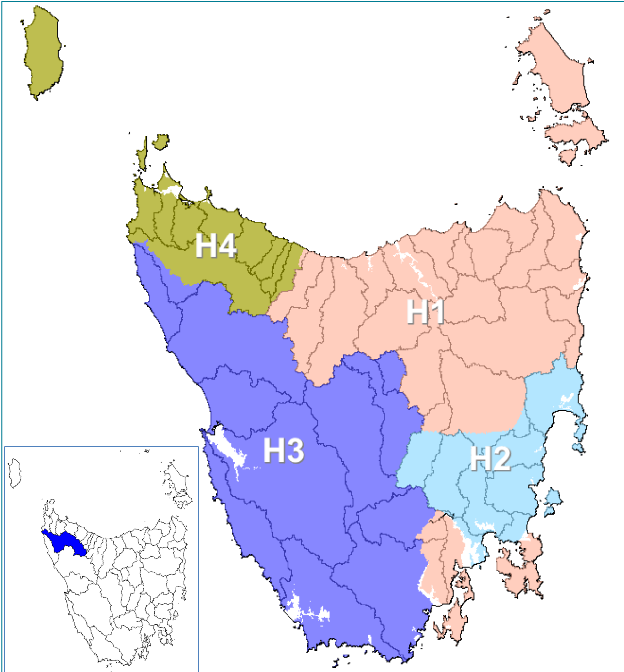
Figure 2. Hydrological regions (Hughes, 1987) and topographic catchments (Arthur highlighted on inset).
