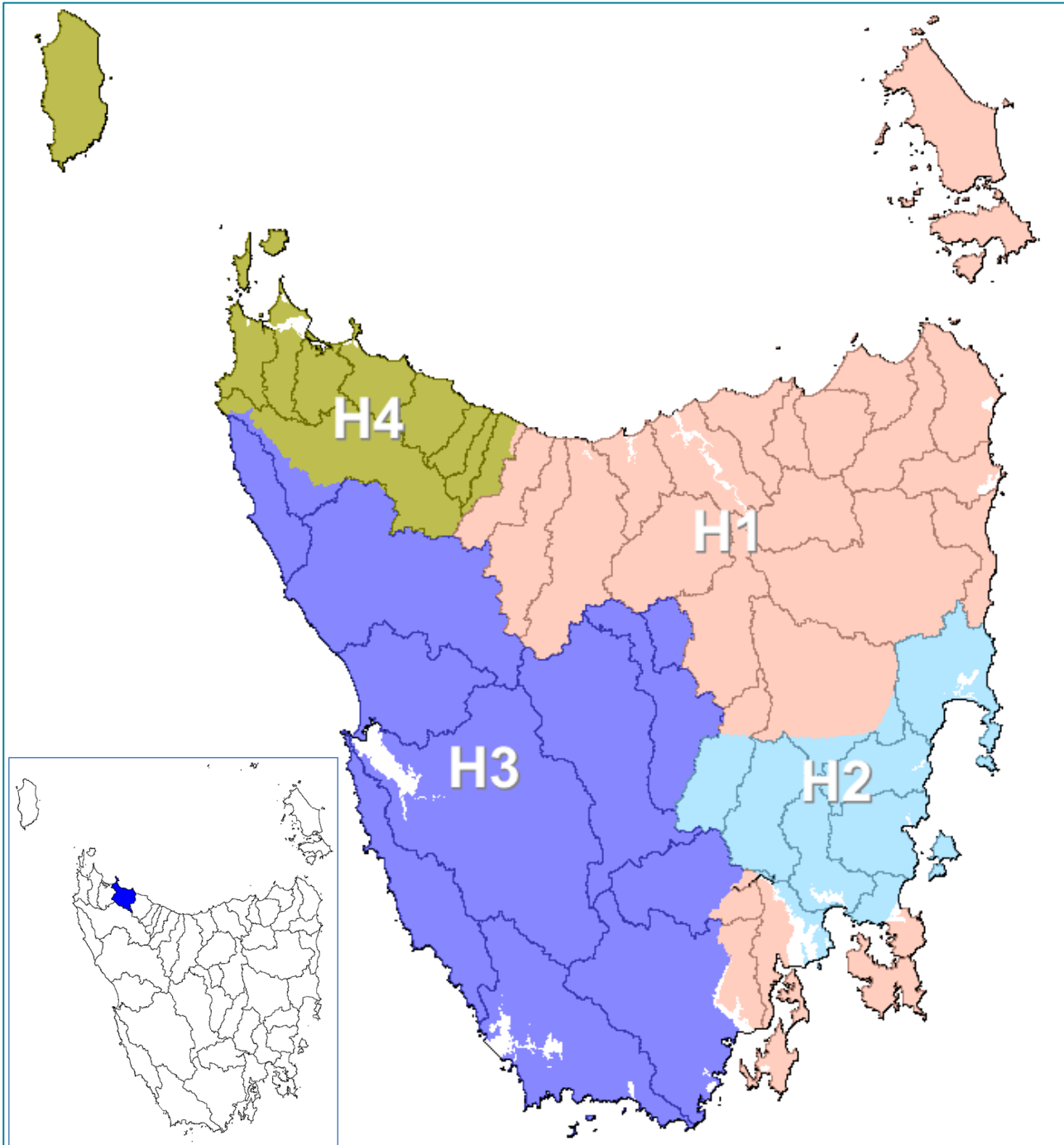
Figure 2. Hydrological regions (Hughes, 1987) and topographic catchments (Black-Detention highlighted on inset).
