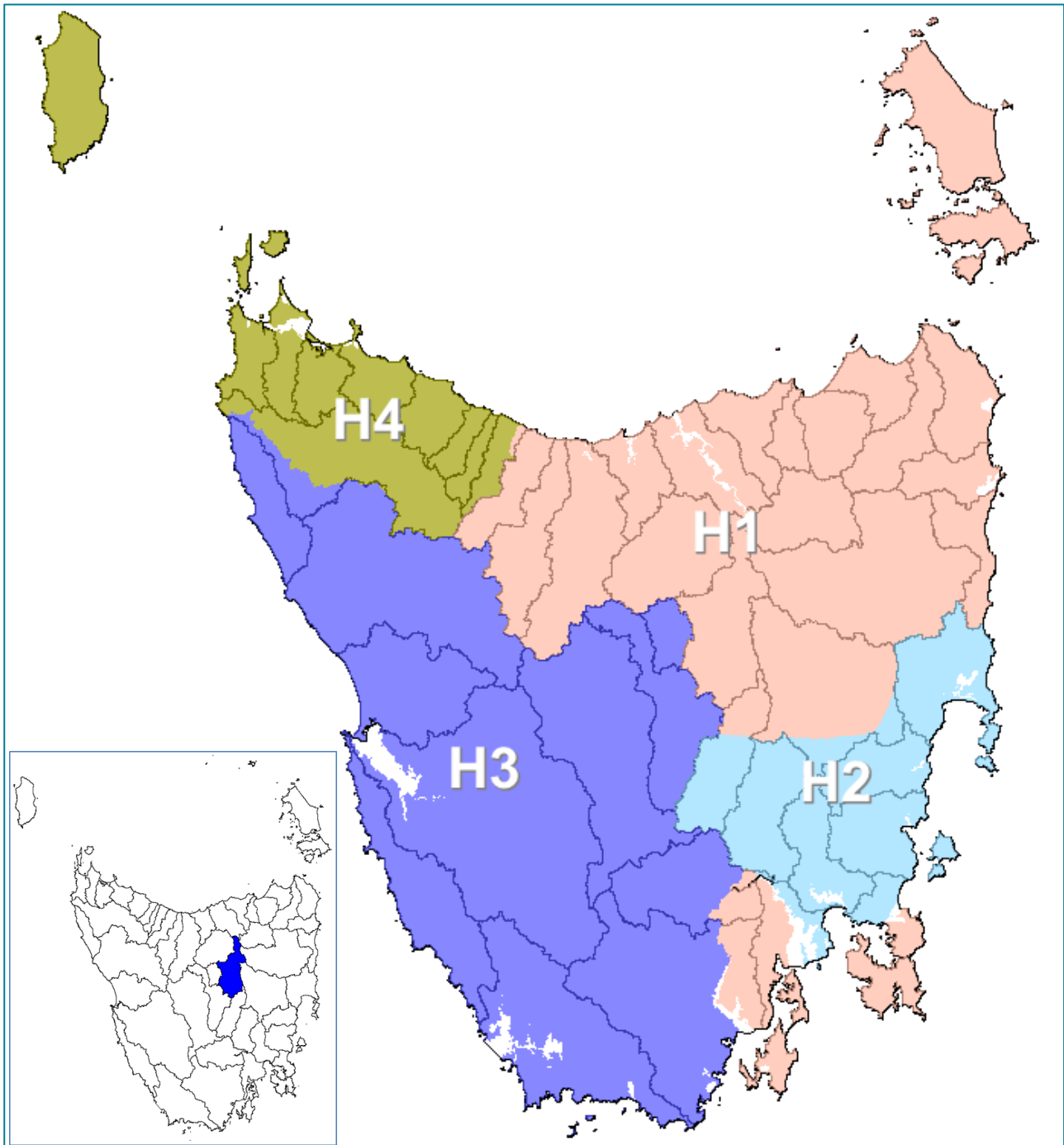
Figure 2. Hydrological regions (Hughes, 1987) and topographic catchments (Brumbys-Lake highlighted on inset).
