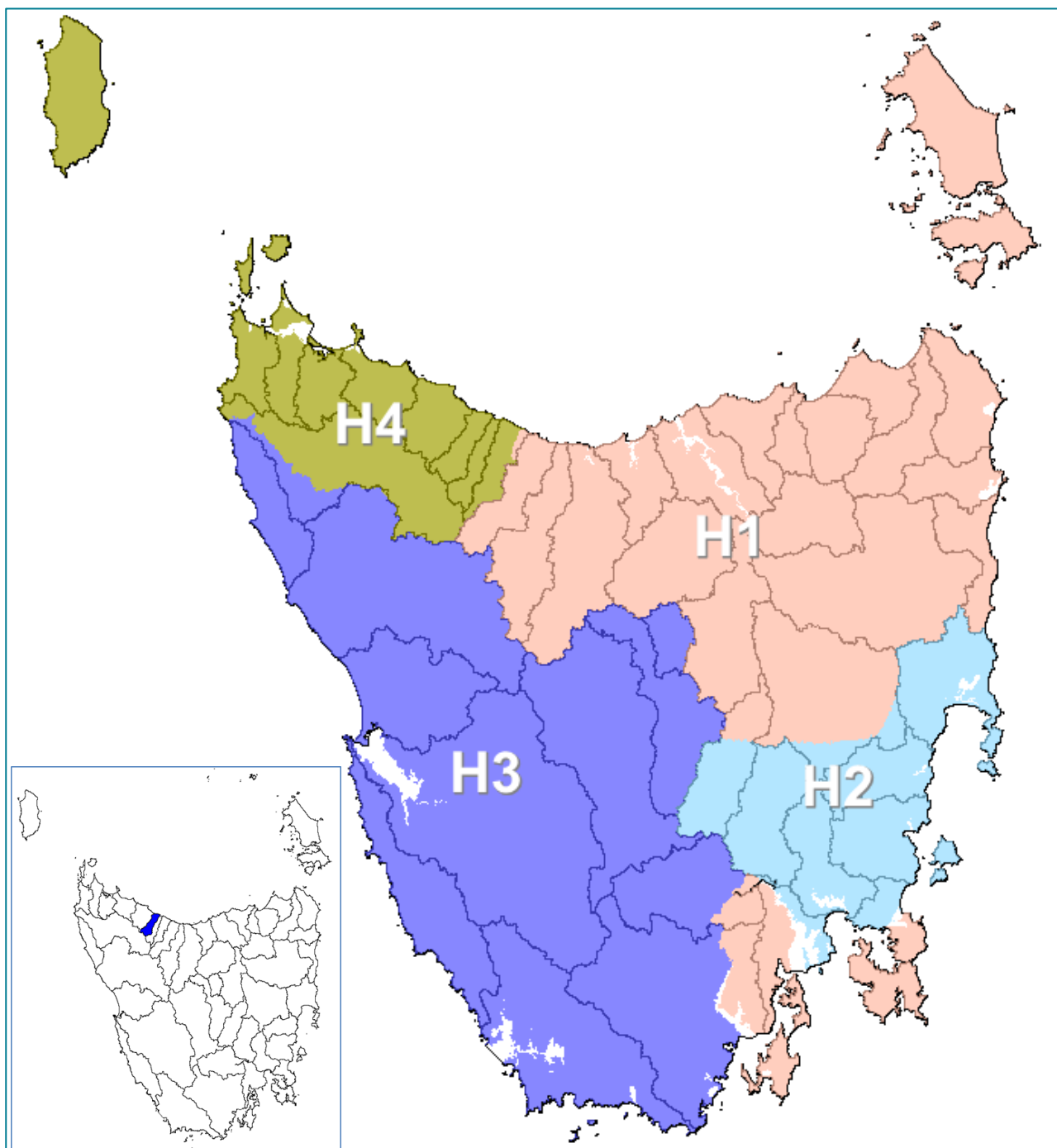
Figure 2. Hydrological regions (Hughes, 1987) and topographic catchments (Cam highlighted on inset).
