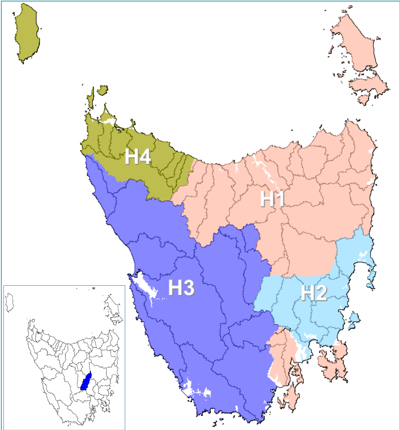
Figure 2. Hydrological regions (Hughes, 1987) and topographic catchments (Clyde highlighted on inset).
