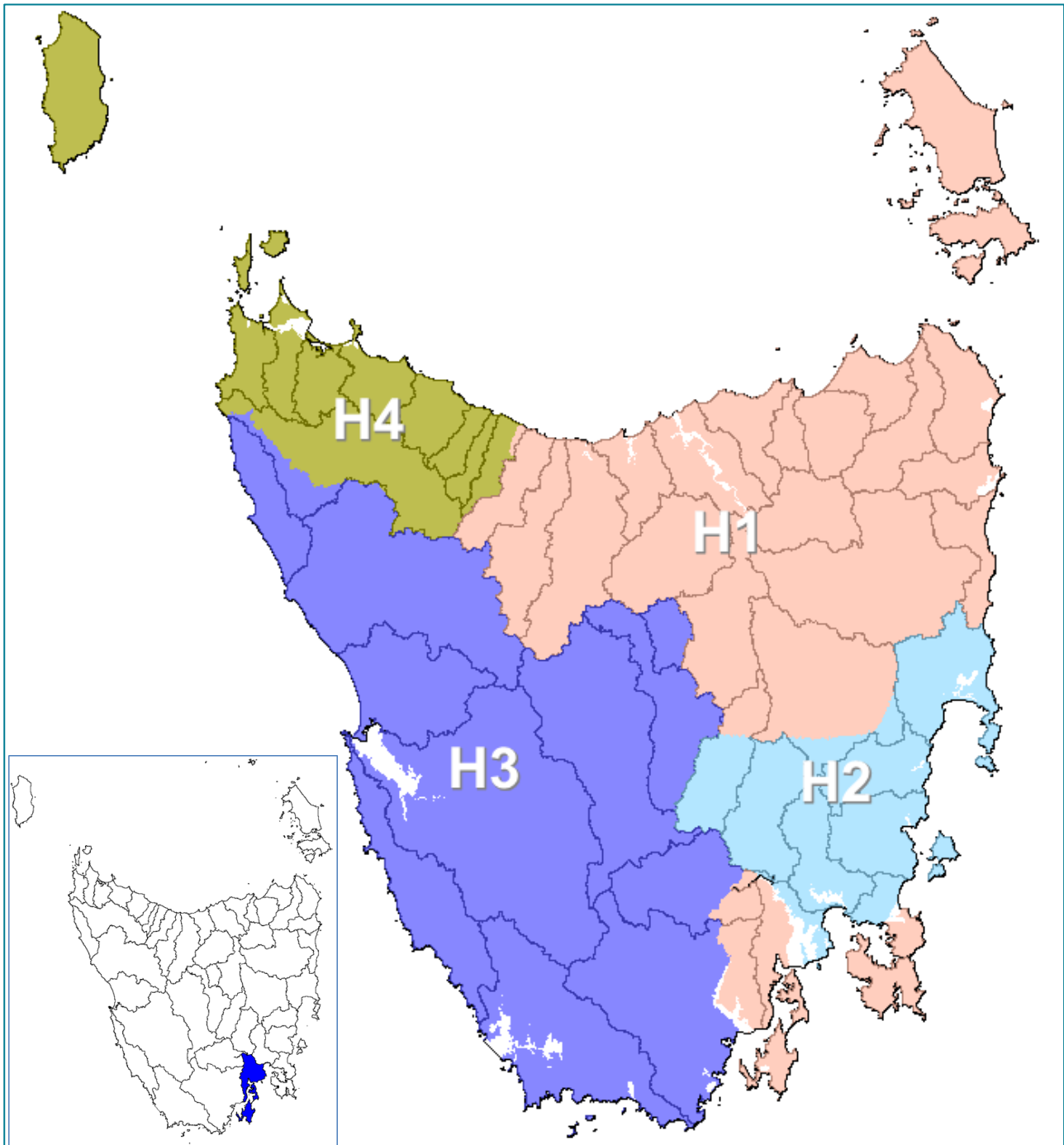
Figure 2. Hydrological regions (Hughes, 1987) and topographic catchments (Derwent Estuary-Bruny highlighted on inset).
