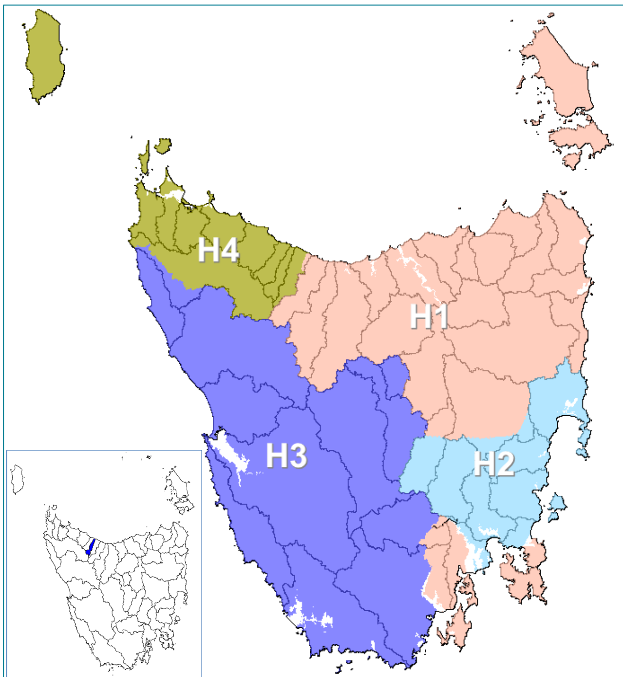
Figure 2. Hydrological regions (Hughes, 1987) and topographic catchments (Emu highlighted on inset).
