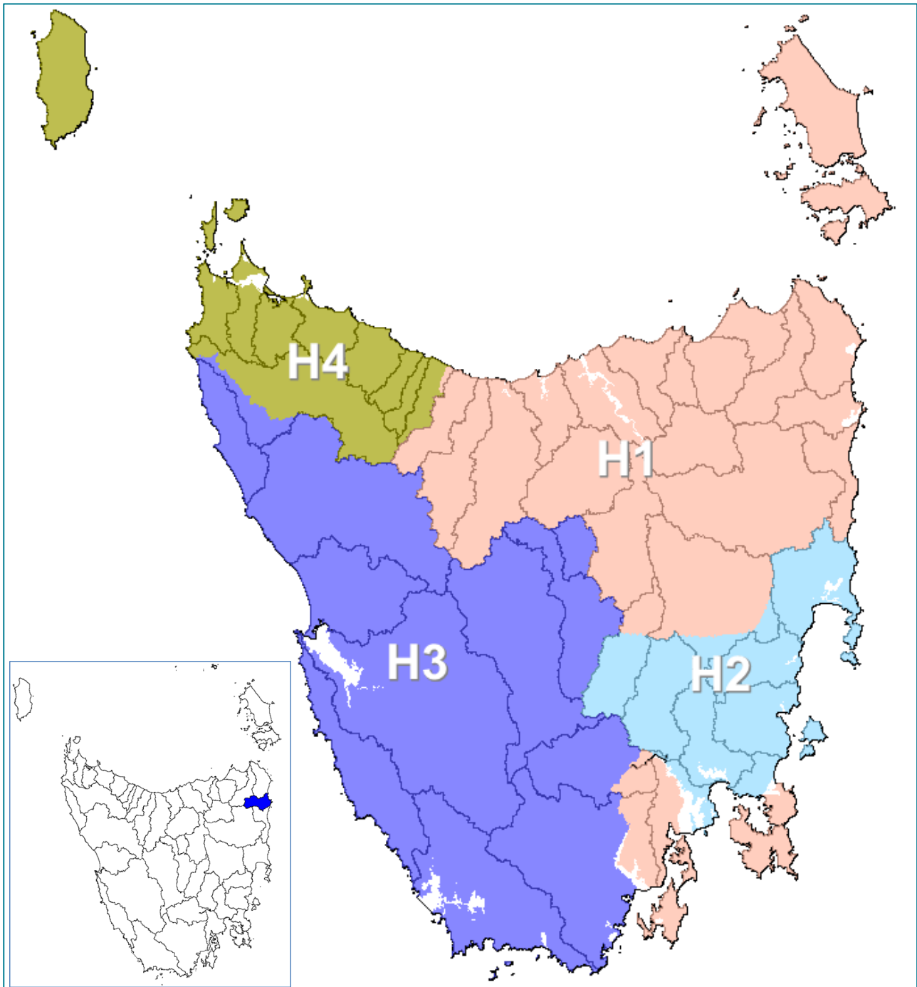
Figure 2. Hydrological regions (Hughes, 1987) and topographic catchments (George highlighted on inset).
