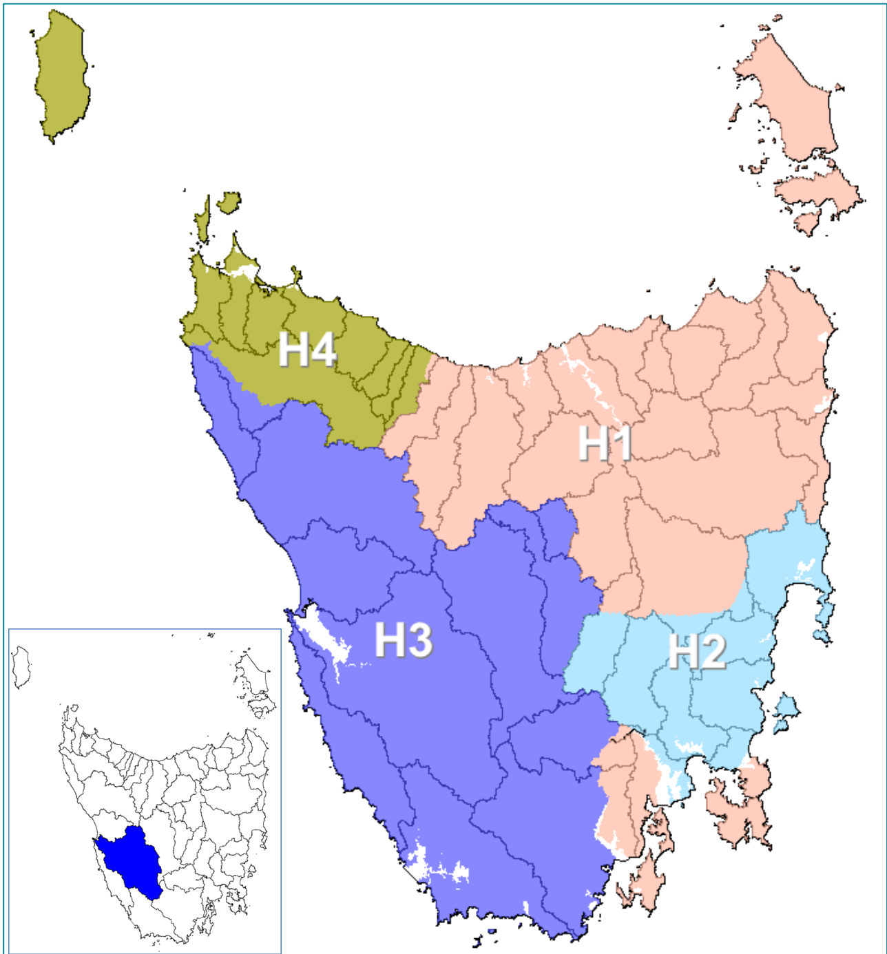
Figure 2. Hydrological regions (Hughes, 1987) and topographic catchments (Gordon-Franklin highlighted on inset).
