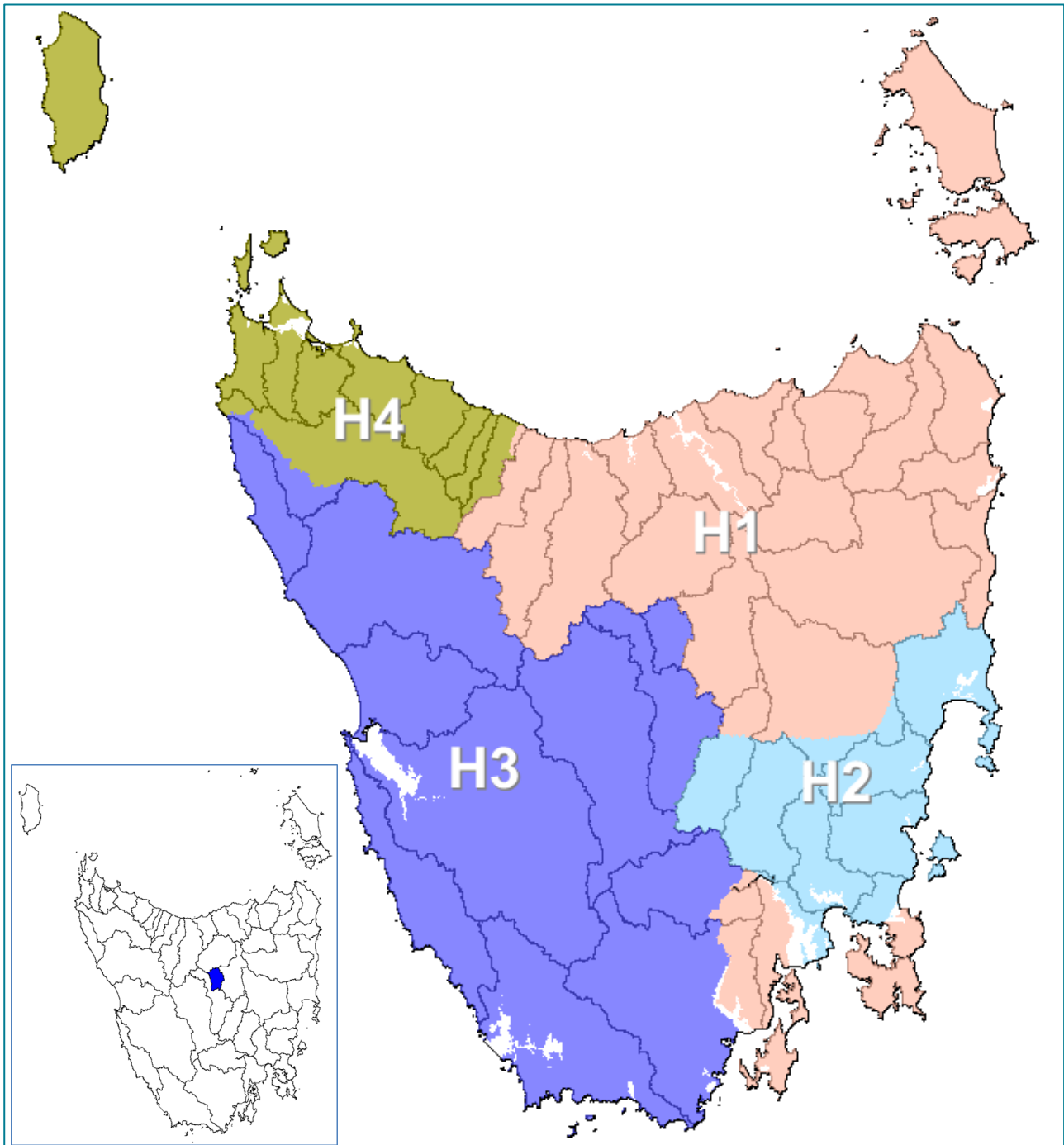
Figure 2. Hydrological regions (Hughes, 1987) and topographic catchments (Great Lake highlighted on inset).
