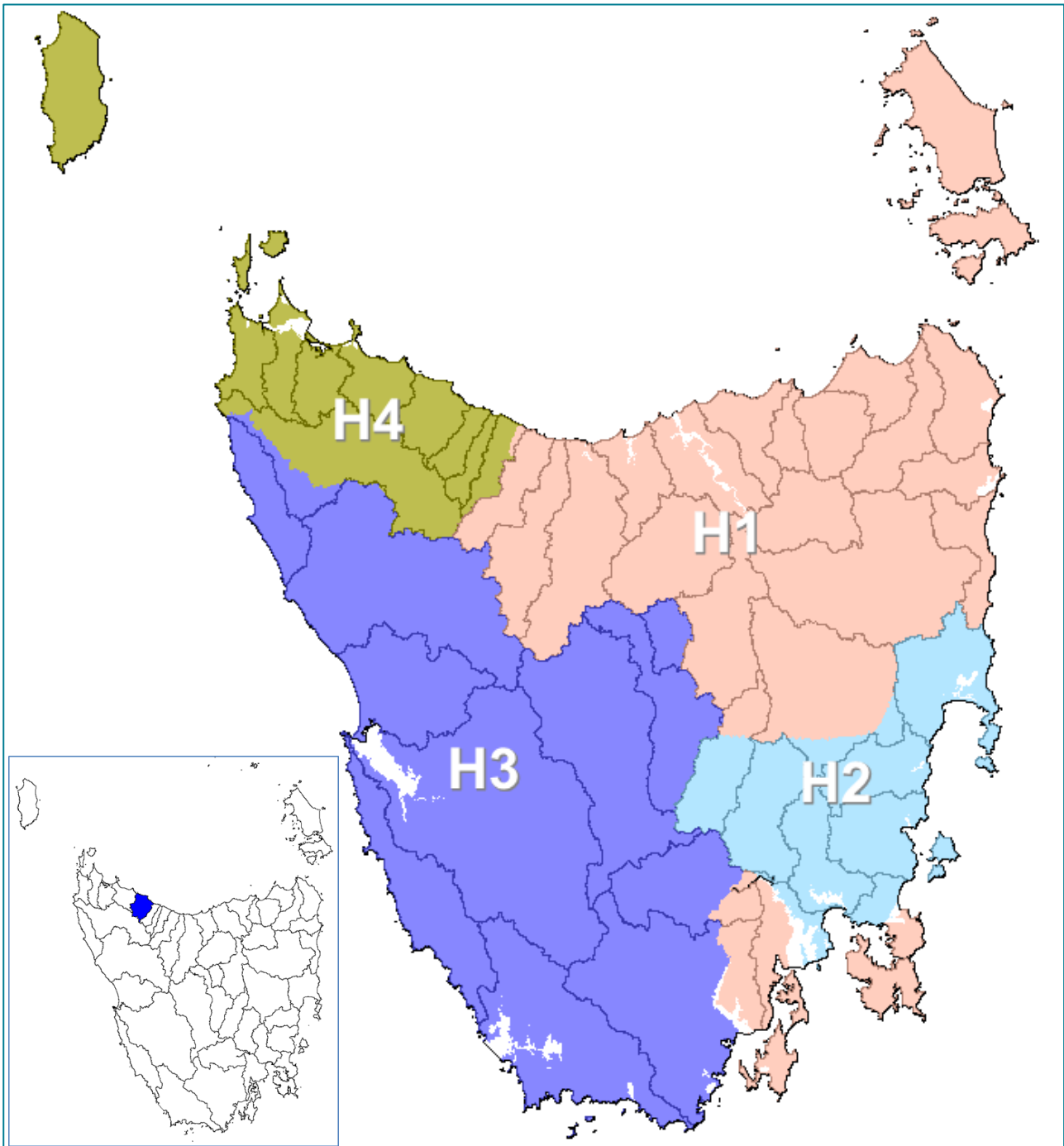
Figure 2. Hydrological regions (Hughes, 1987) and topographic catchments (Inglis-Flowerdale highlighted on inset).
