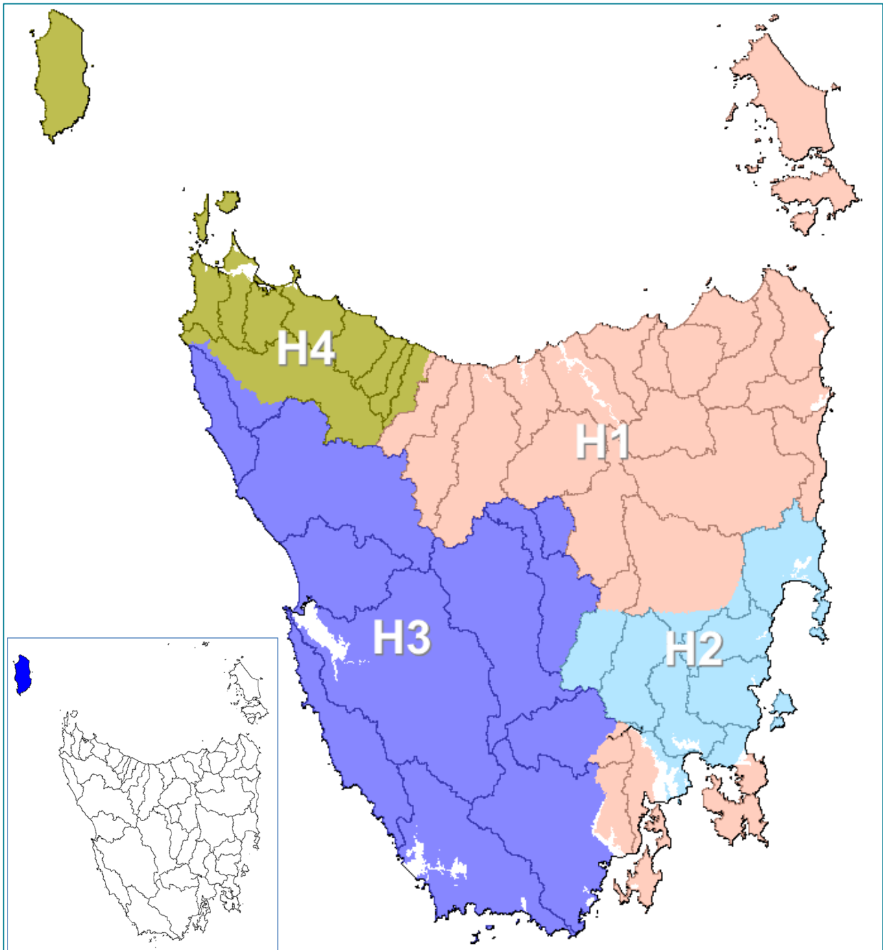
Figure 2. Hydrological regions (Hughes, 1987) and topographic catchments (King Island highlighted on inset).
