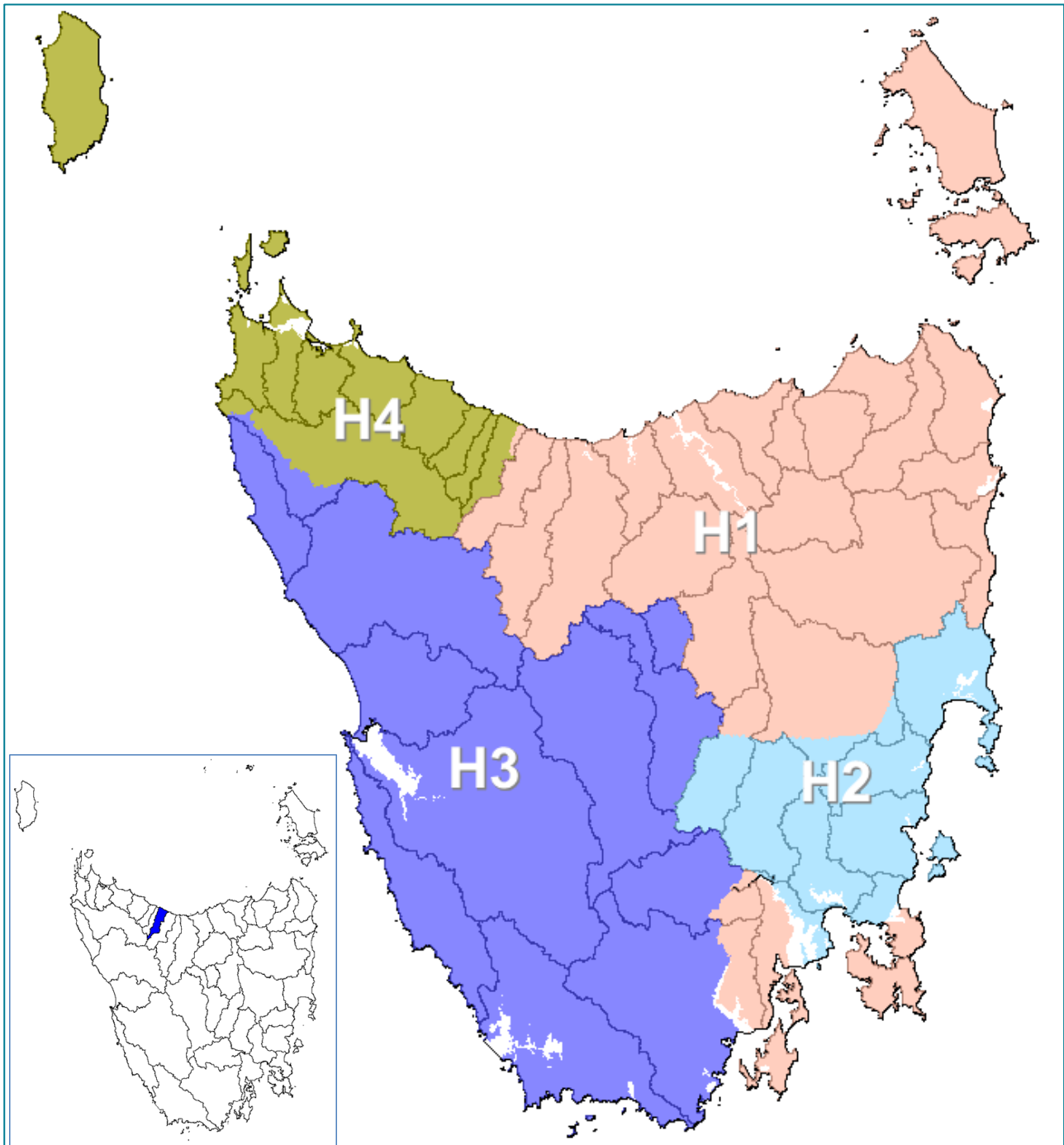
Figure 2. Hydrological regions (Hughes, 1987) and topographic catchments (Leven highlighted on inset).
