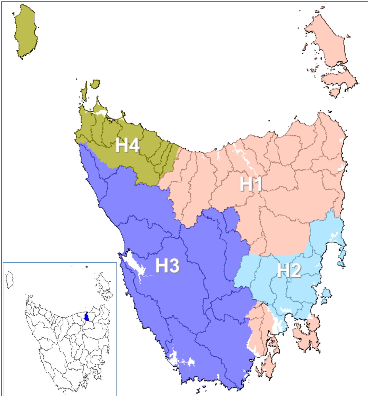
Figure 2. Hydrological regions (Hughes, 1987) and topographic catchments (Little Forester highlighted on inset).
