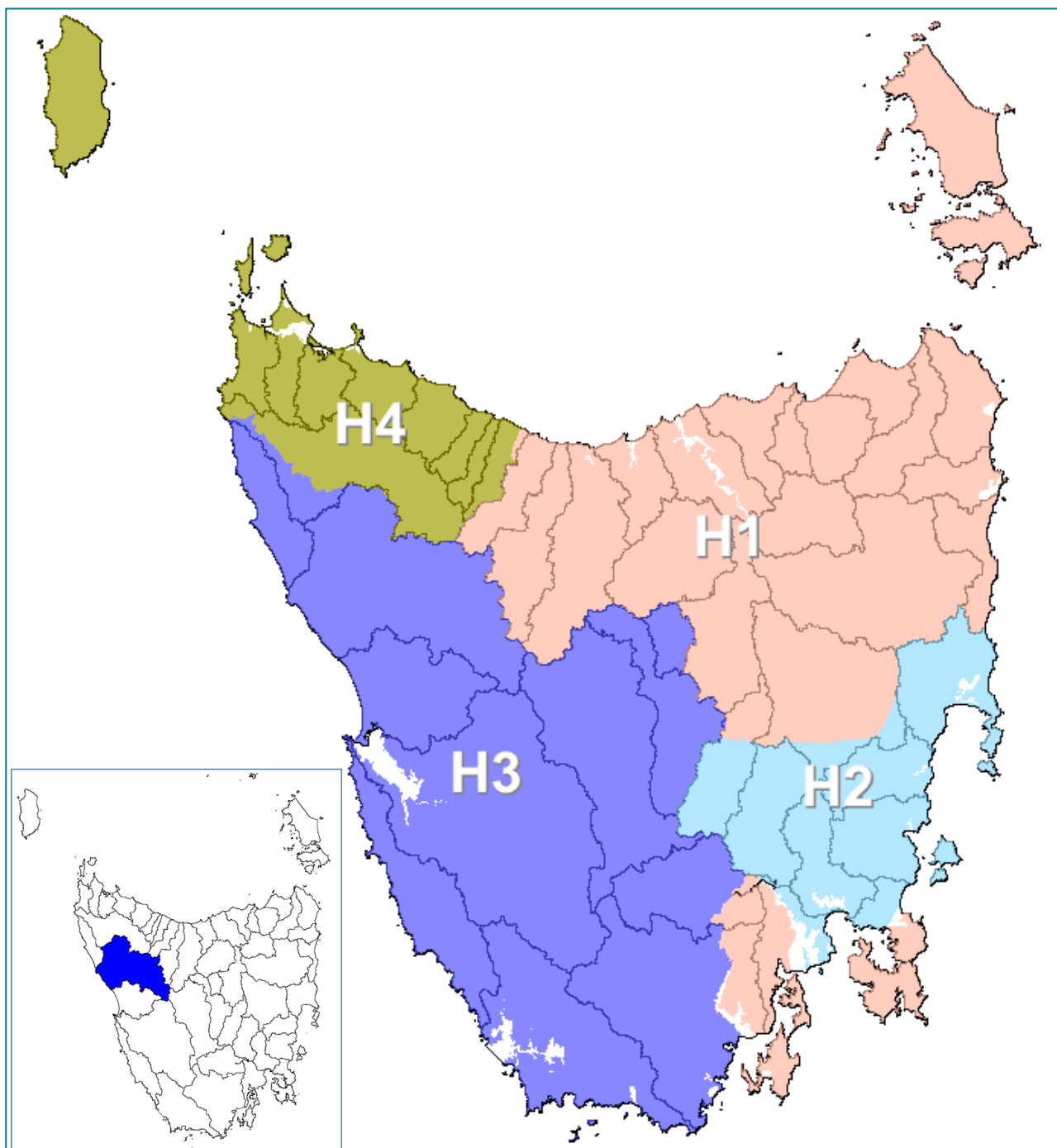
Figure 2. Hydrological regions (Hughes, 1987) and topographic catchments (Pieman highlighted on inset).
