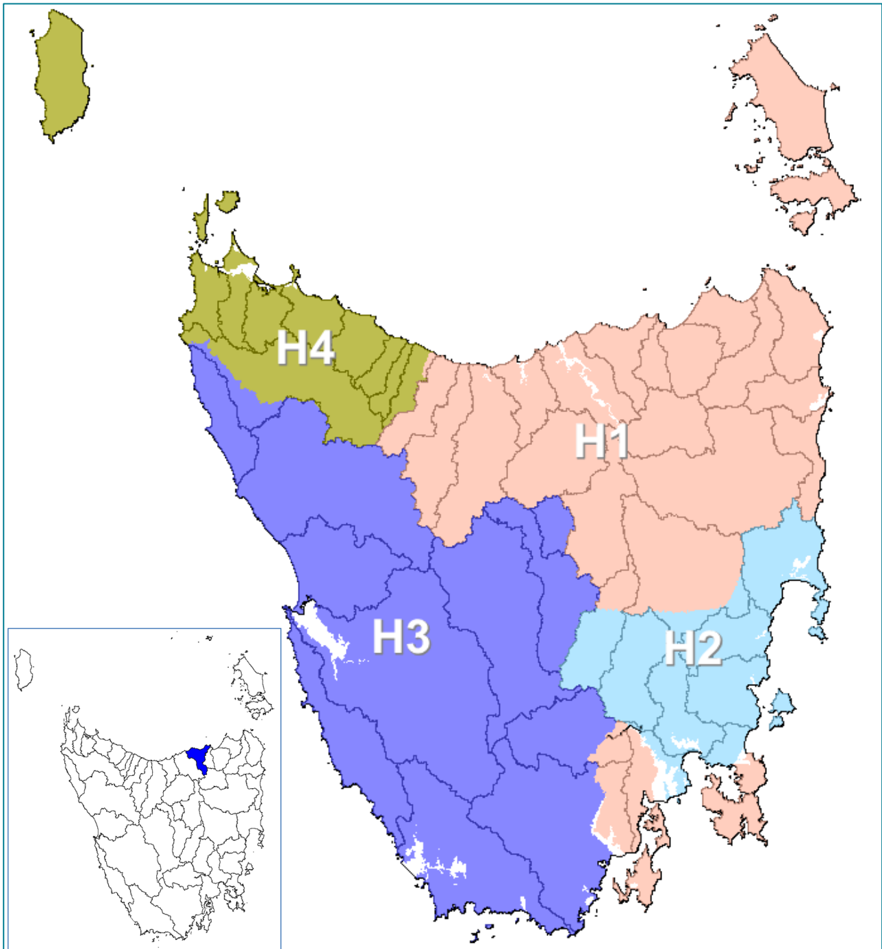
Figure 2. Hydrological regions (Hughes, 1987) and topographic catchments (Pipers highlighted on inset).
