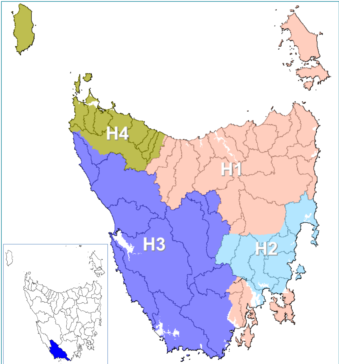
Figure 2. Hydrological regions (Hughes, 1987) and topographic catchments (Port Davey highlighted on inset).
