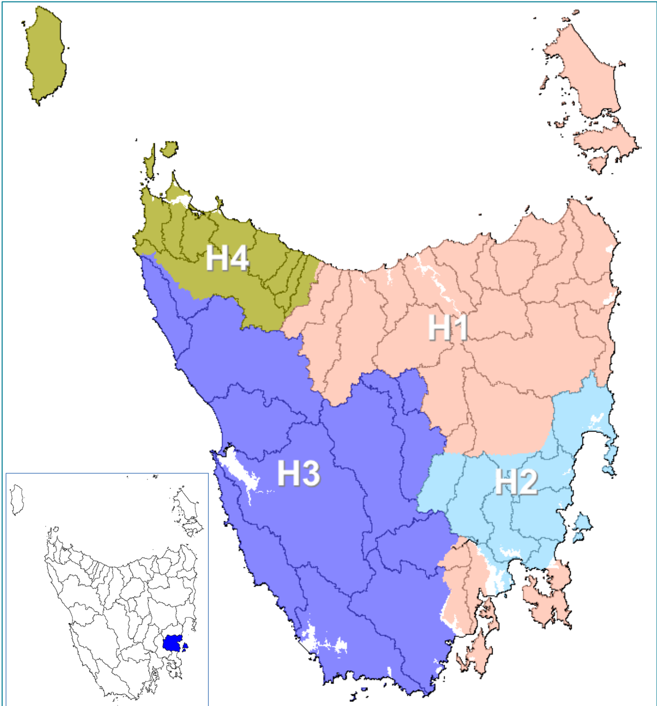
Figure 2. Hydrological regions (Hughes, 1987) and topographic catchments (Prosser highlighted on inset).
