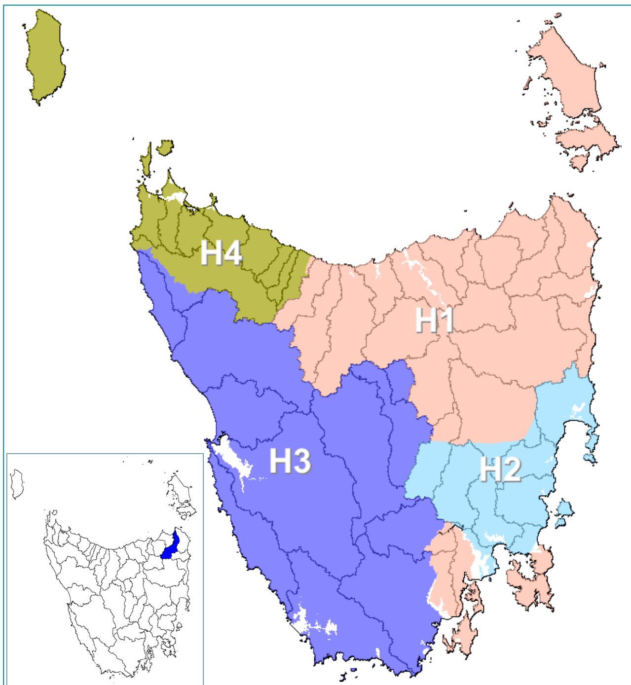
Figure 2. Hydrological regions (Hughes, 1987) and topographic catchments (Ringarooma highlighted on inset).
