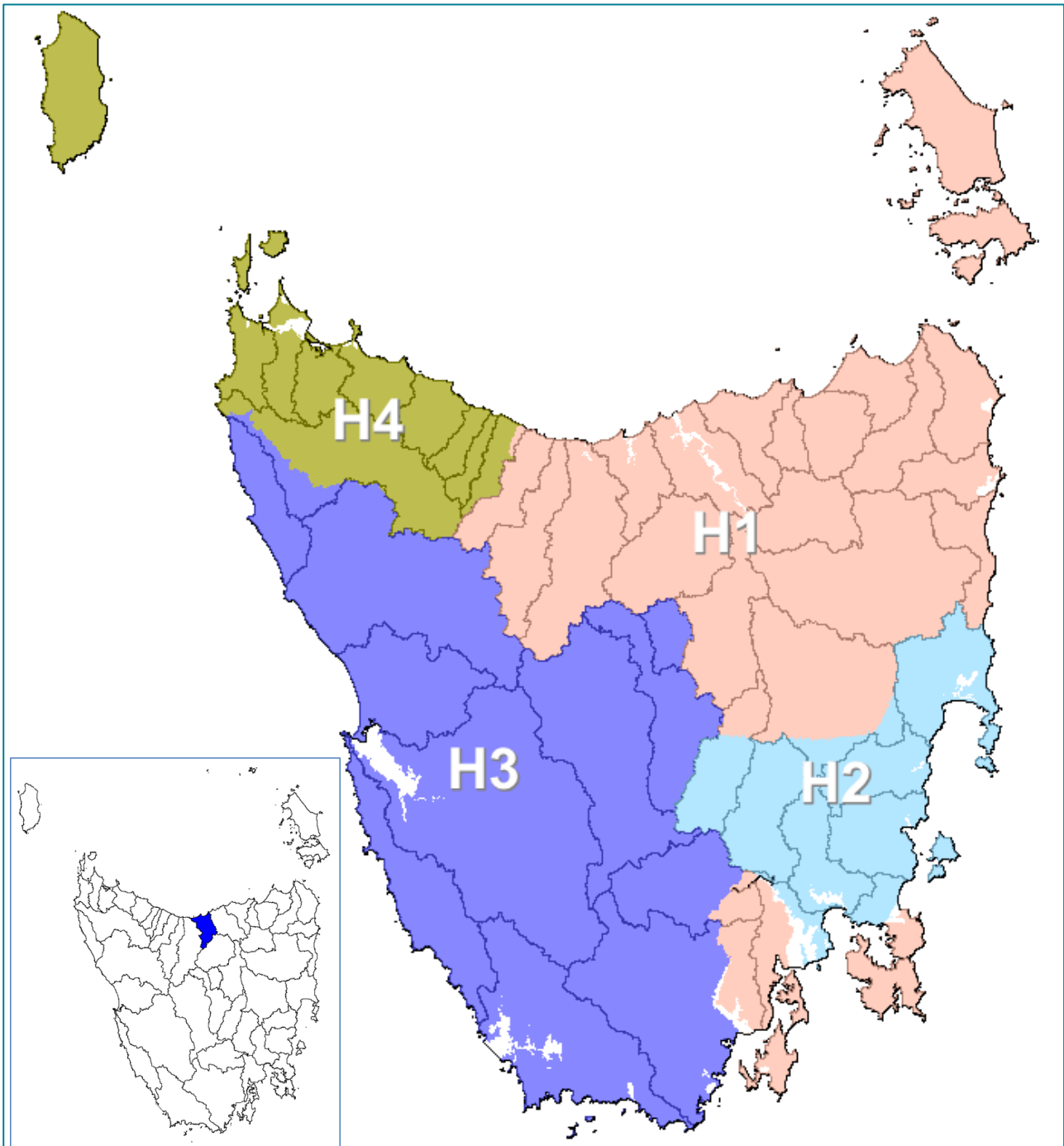
Figure 2. Hydrological regions (Hughes, 1987) and topographic catchments (Rubicon highlighted on inset).
