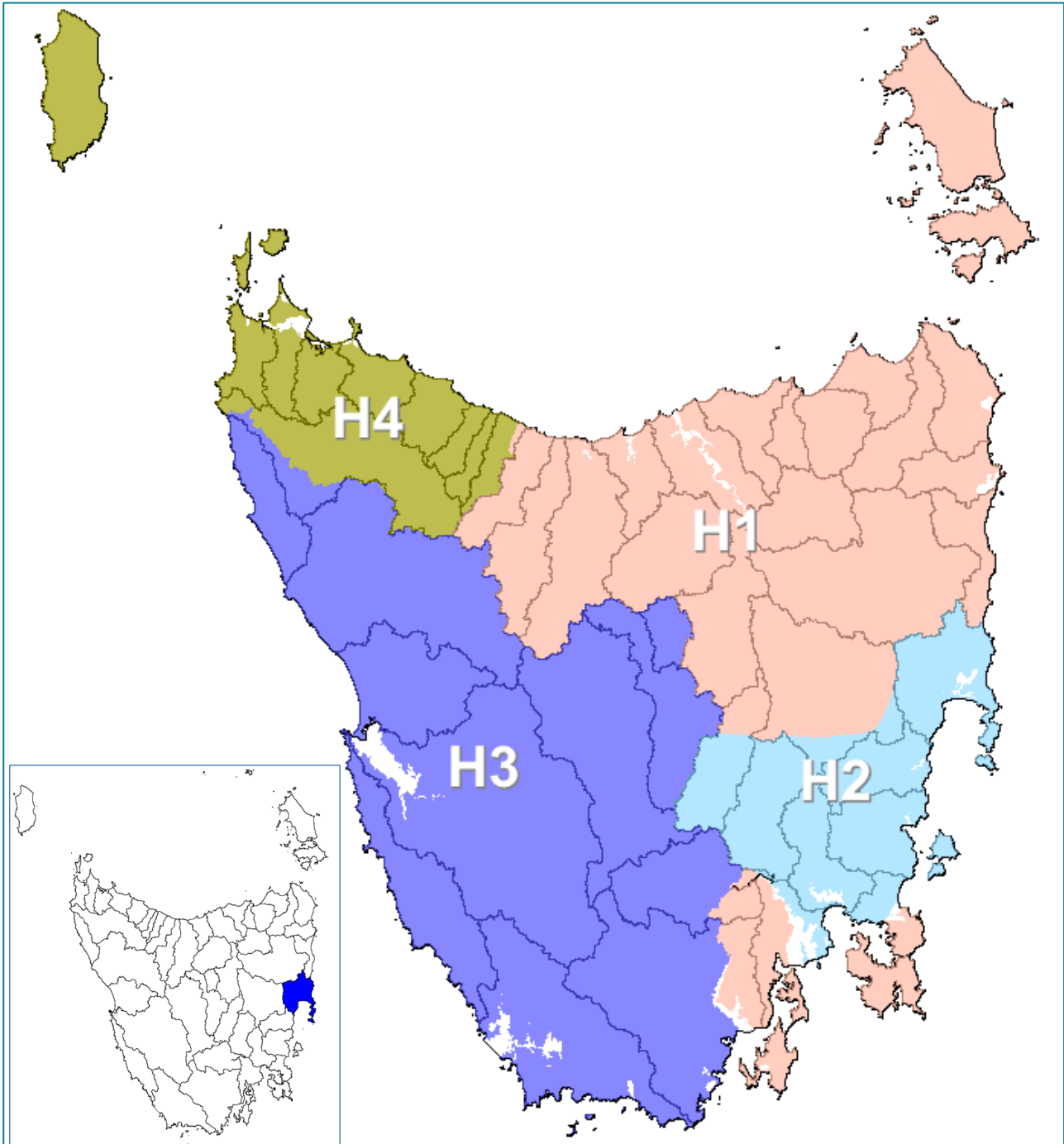
Figure 2. Hydrological regions (Hughes, 1987) and topographic catchments (Swan-Apsley highlighted on inset).
