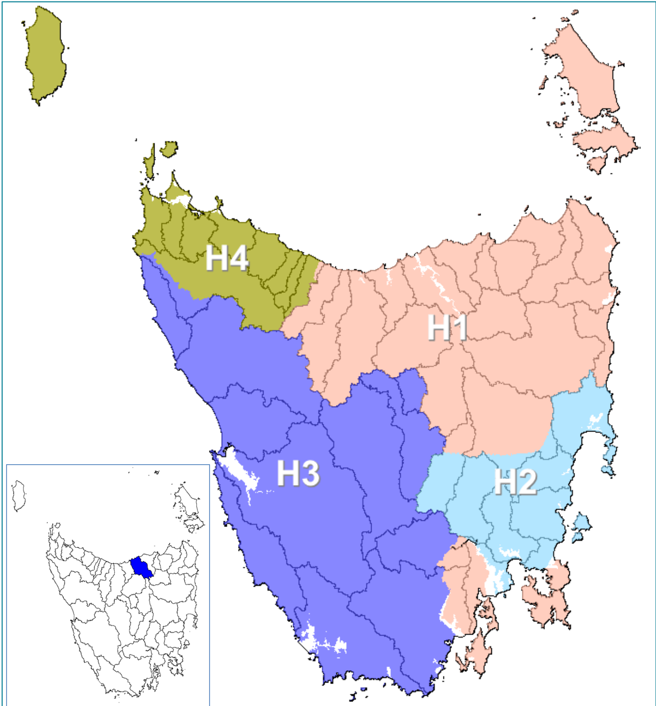
Figure 2. Hydrological regions (Hughes, 1987) and topographic catchments (Tamar Estuary highlighted on inset).
