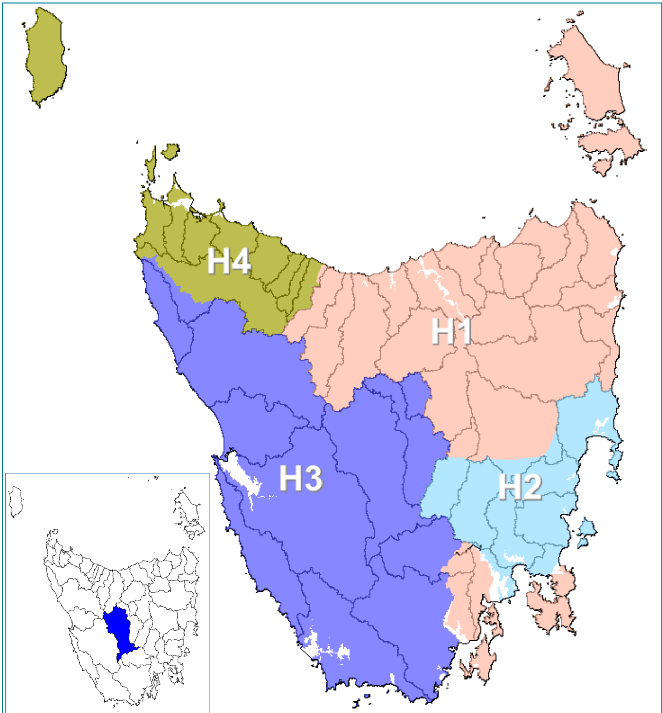
Figure 2. Hydrological regions (Hughes, 1987) and topographic catchments (Upper Derwent highlighted on inset).
