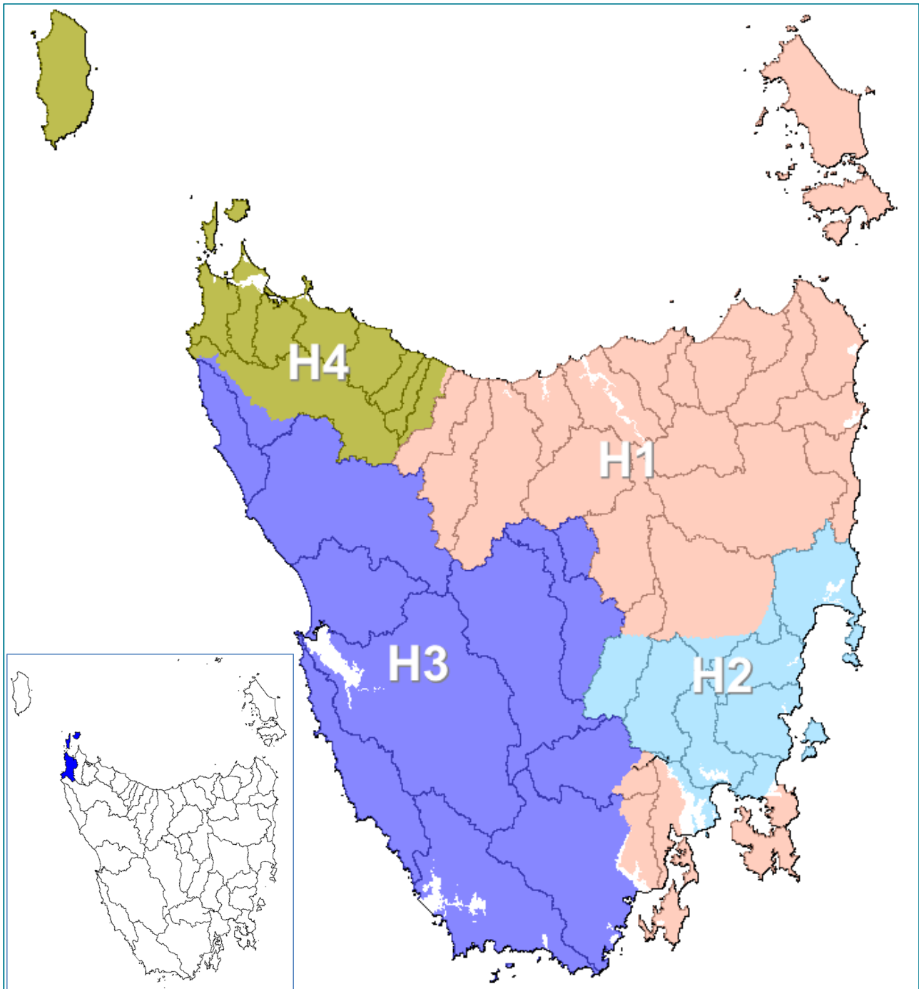
Figure 2. Hydrological regions (Hughes, 1987) and topographic catchments (Welcome highlighted on inset).
