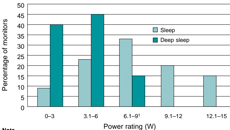
Figure 4 Sleep mode ratings for monitors on the ENERGY STAR database, 1 July 2000
