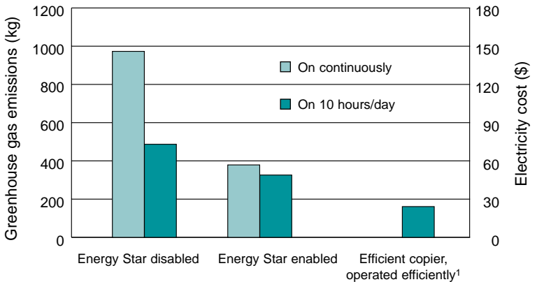
Figure 5 Annual greenhouse gas emissions and electricity consumption from photocopiers (50 cpm, 1,000 copies/day)
