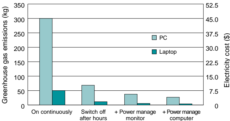
Figure 3 Annual greenhouse gas emissions and electricity consumption for PCs and laptops
