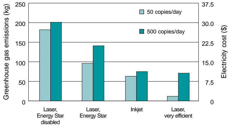
Figure 7 Annual electricity-based greenhouse gas emissions and electricity consumption from fax machines
